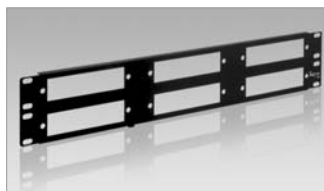
Rack Mount Blank Patch Panel ICFORPP1RM 3-Panel, 1 RMS, For 3 Cassettes ICFORPP2RM 6-Panel, 2 RMS, For 6 Cassettes
